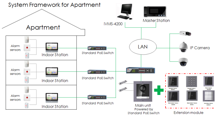
System Framework for Apartment
